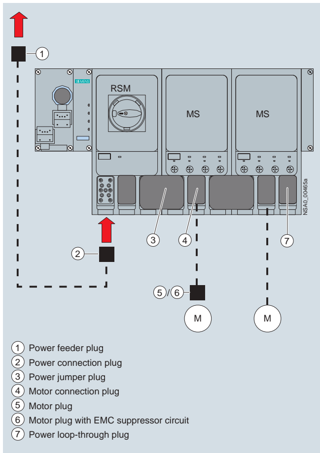
Infeed on the RSM isolator module
