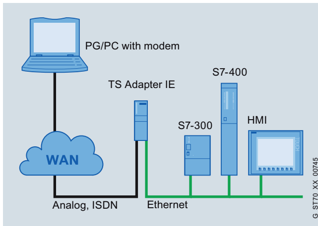
Teleservice with TS Adapter IE
