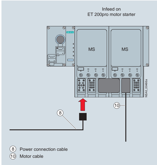
Infeed on the ET 200pro motor starter
